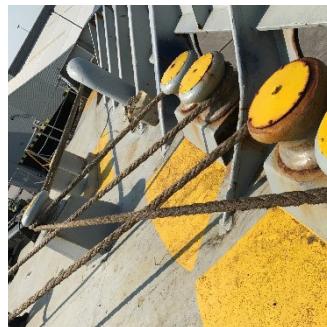
Rope-on-rope abrasion and poorly maintained mooring system
